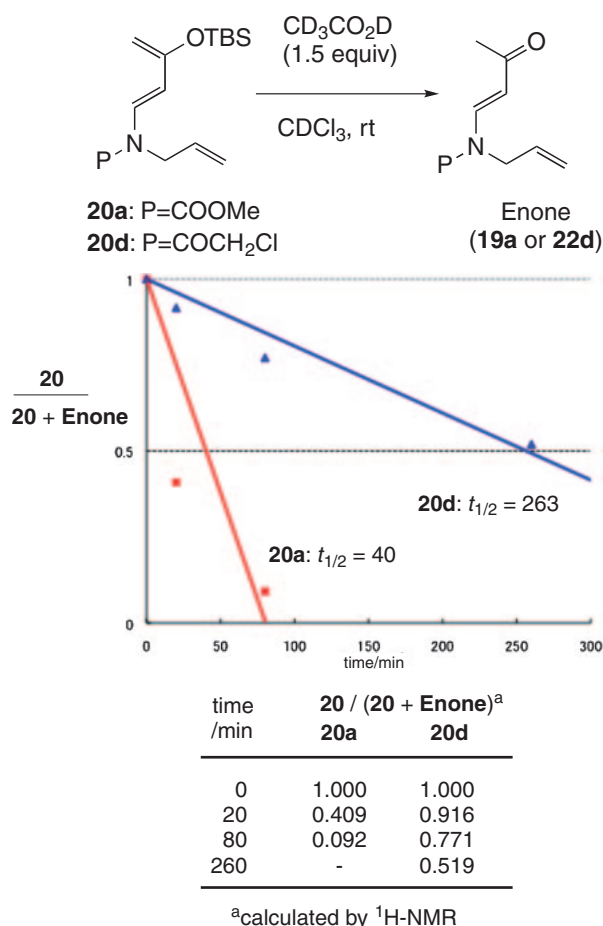
Figure 4. Decomposition experiments with 20a and 20d .
