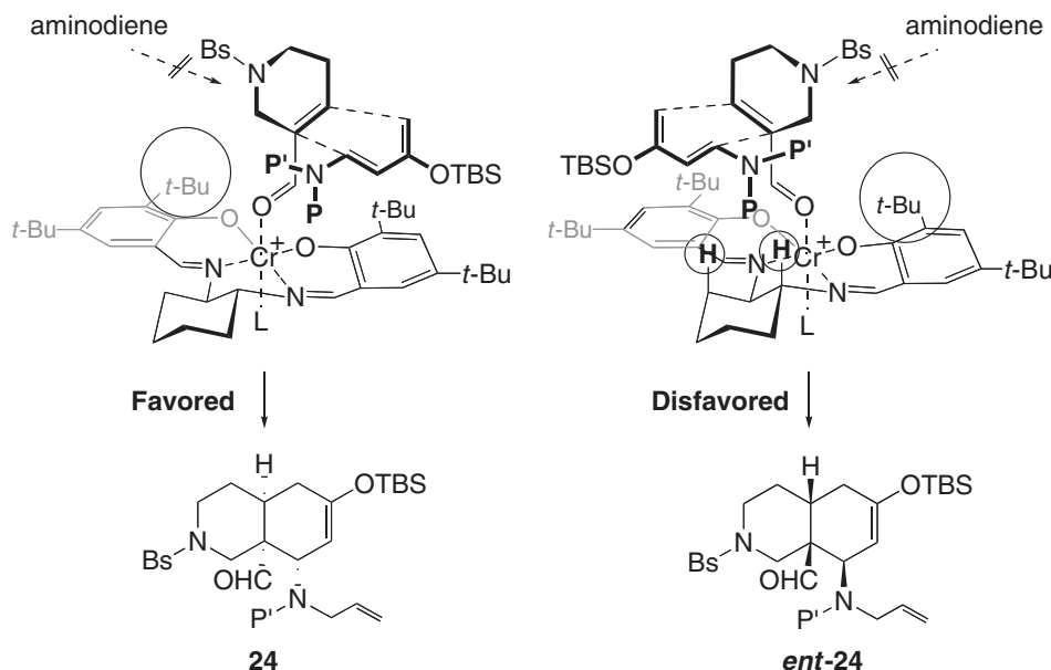
Figure 3. Plausible transition state in the Diels–Alder reaction.
