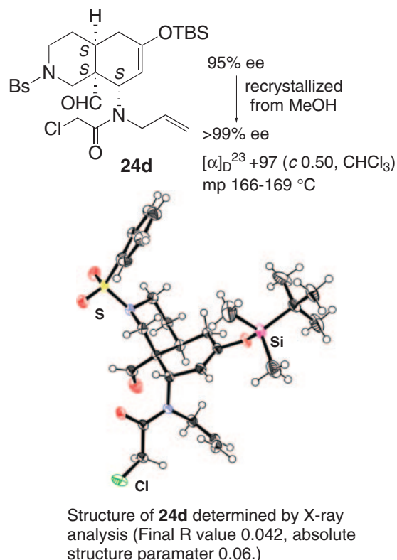
Figure 2. Determination of relative and absolute stereochemistry.
