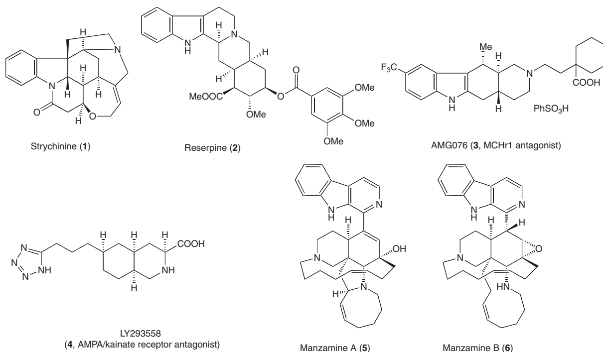
Figure 1. Natural and unnatural compounds with a hydroisoquinoline skeleton.
